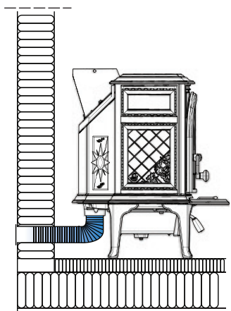
Fig. 6a Through an outside wall
