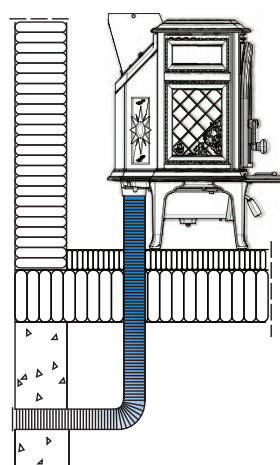
Fig. 6d Indirectly through an outside wall
