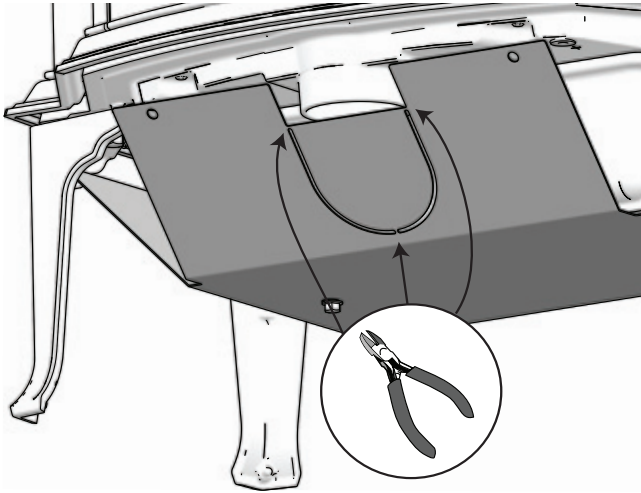
Fig. 7a Mounting of external air supply connection
