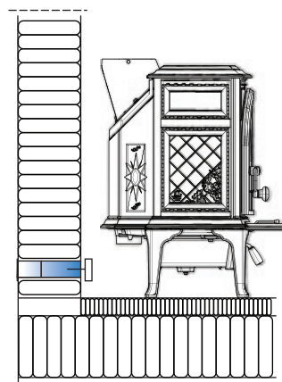
Fig. 6d Indirectly through an outside wall
