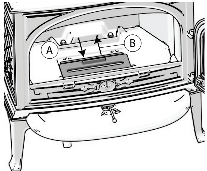
Fig. 12 Ash grate
