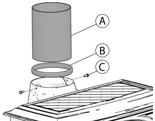
Fig. 5 Assembling the flue pipe
