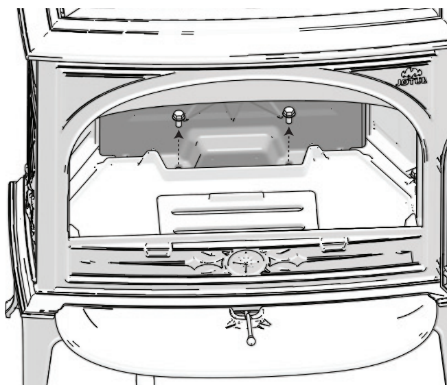
Fig. 18a Replacing the rear burn plate
