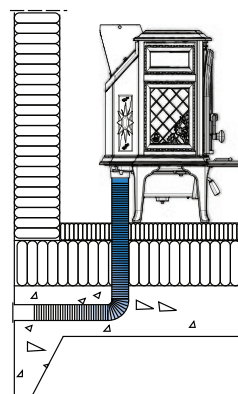
Fig. 6b Through the floor and ground plate
