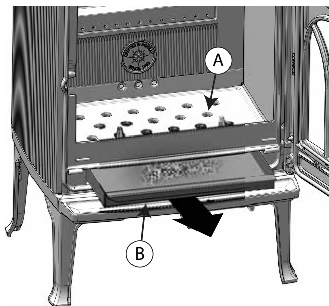
Fig. 13 Ash grate
