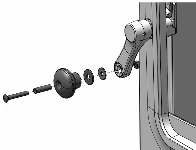
Fig. 3b Installation of the door handle (F 205 V2 IT - modern)
