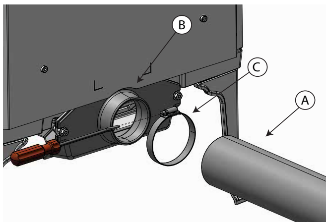
Fig. 6 Instal external air supply
