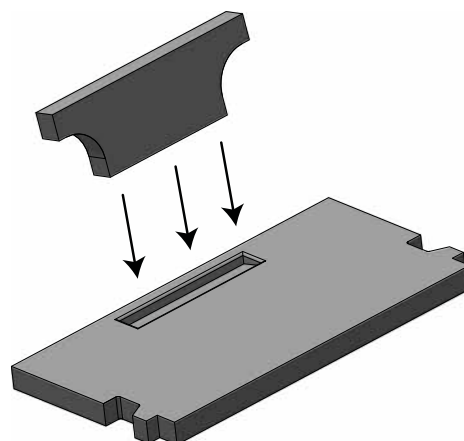
Fig. 17 Placement of the upper exhaust deflector
