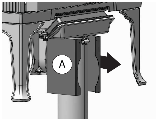
Fig. 8 Installation of cover for outdoor air (Optional equipment - 50061978)
