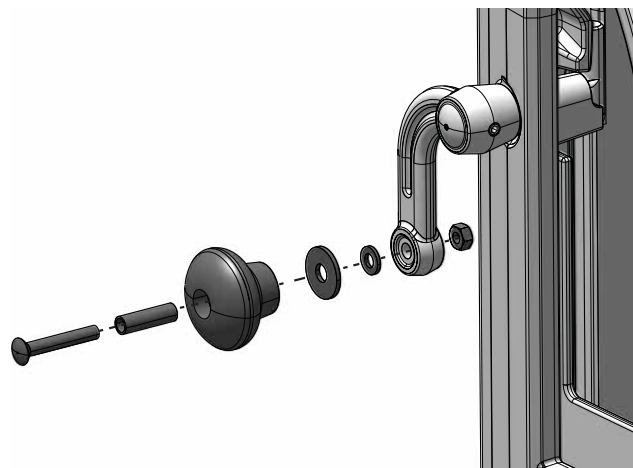
Fig. 3a Installation of the door handle (F 200 HE+ - classic)
