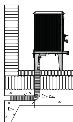
Fig. 5b Through the floor and ground plate
