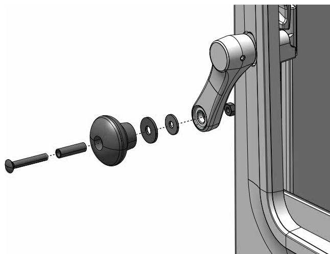
Fig. 3b Installation of the door handle (F 205 HE+ - modern)
