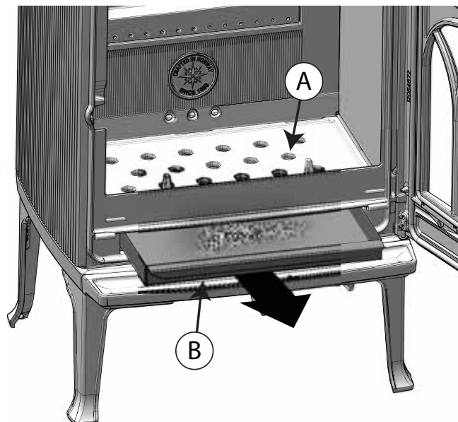
Fig. 13 Ash grate
